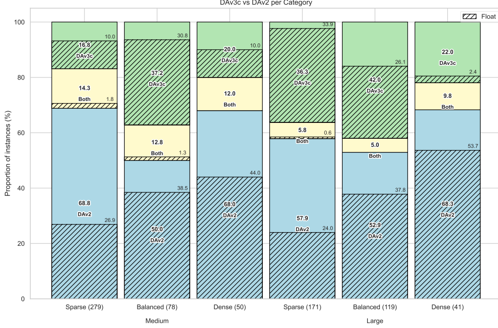
Fig. 5: Performance comparison between DAv3c and DAv2 across size–density groups using the same visualization scheme as Figure 2.
