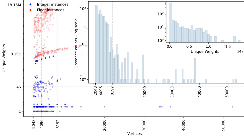
Fig. 1: Relationship between edge-weight representation and the number of unique edge weights across benchmark instances. Floating-point instances generally exhibit substantially higher weight diversity than integer-weighted instances.
