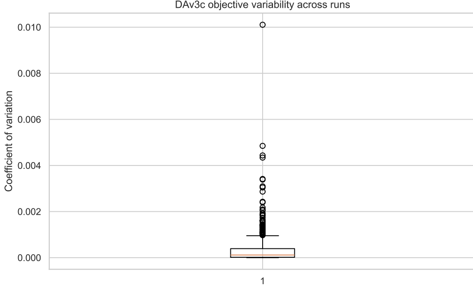
Fig. B2: Distribution of coefficient of variation (CV) values across all evaluated instances. CV values are computed from the objective values obtained over five independent runs for each instance, measuring the variability of solver performance across runs.
