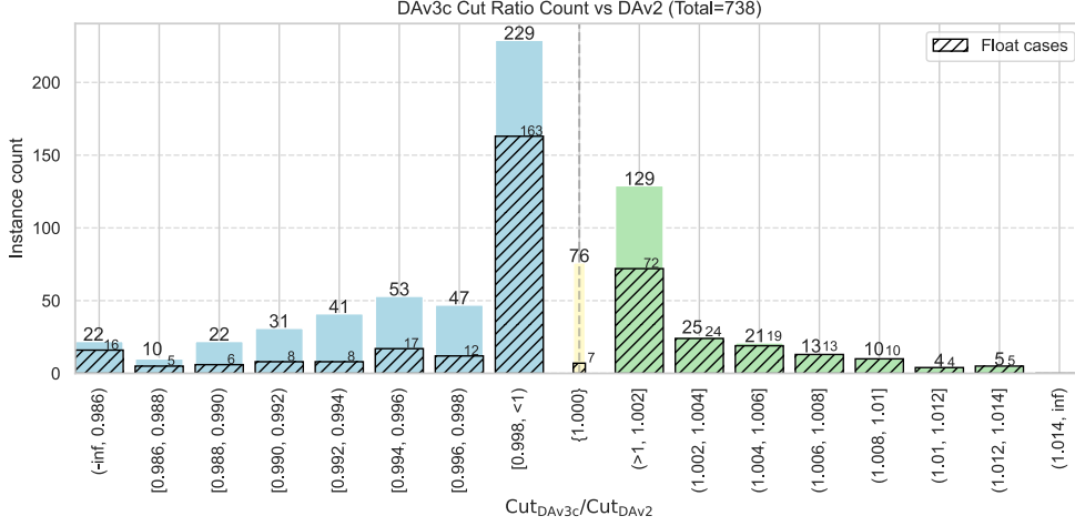
Fig. H6: Distribution of cut-value ratios for DAv3c relative to DAv2 using the same ratio definition as Figure 3.
