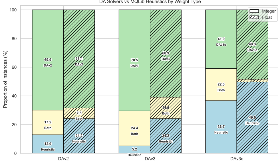
Fig. 6: Aggregate performance comparison of DAv2, DAv3, and DAv3c against the category-specific MQLib heuristic baselines for integer-weighted and non-integer-weighted instances.
