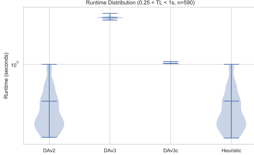
Fig. A1: Violin plot of solver runtime distributions for instances with baseline time limits (TL) satisfying 0.25 < TL < 1 seconds. Wider regions indicate a higher concentration of instances at the corresponding runtime values. The total number of instances is reported in the plot title.
