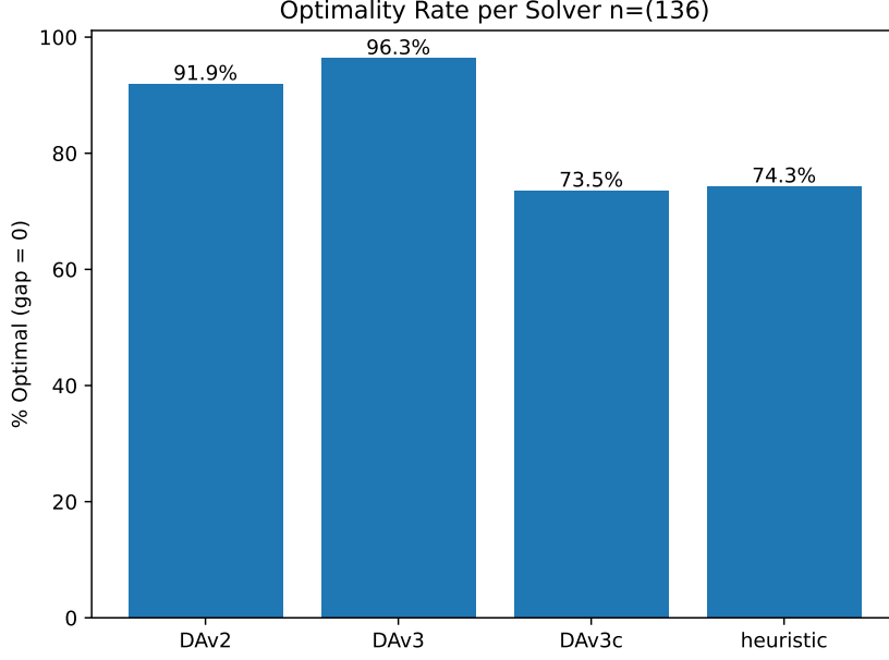
Fig. 7: Optimality rate (%) of each solver on the common subset of 136 bipartite instances with non-negative edge weights. Optimality rate is defined as the proportion of instances for which the solver attains the true optimal cut value. The 10 xlarge instances are excluded because DAv2 results are not available for this size category.
