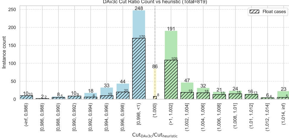
Fig. 3: Distribution of cut-value ratios across all considered instances. The ratio is defined as \text{Cut}_{\text{DAv3c}}/\text{Cut}_{\text{heuristic}} . Values close to 1 indicate near-identical solution quality, while deviations above or below 1 reflect relative improvements or degradations in DAv3c performance compared to the selected heuristic.
