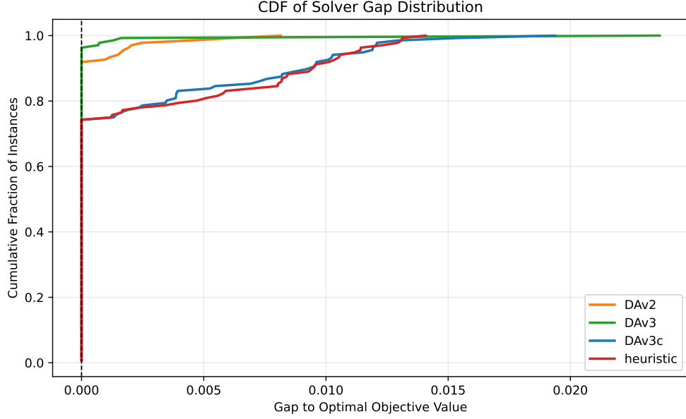
Fig. 8: Empirical cumulative distribution of the relative gap to the true optimal value for bipartite instances with non-negative edge weights. Curves closer to the top-left indicate better solver performance, corresponding to smaller relative gaps across a larger proportion of instances.
