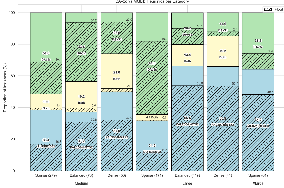
Fig. 2: Performance comparison between DAv3c and the category-selected MQLib heuristics across size–density groups. Green, yellow, and blue denote DAv3c wins, ties, and heuristic wins, respectively. The percentage labels inside each segment indicate the proportion of instances belonging to that outcome within a category, summing to 100% per category. Hatched regions correspond to floating-point-weighted instances, and the associated annotations indicate their proportion relative to the total number of instances in the category.
