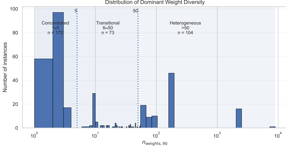
Fig. C3: Distribution of the n_{90} metric across integer-weighted benchmark instances.
