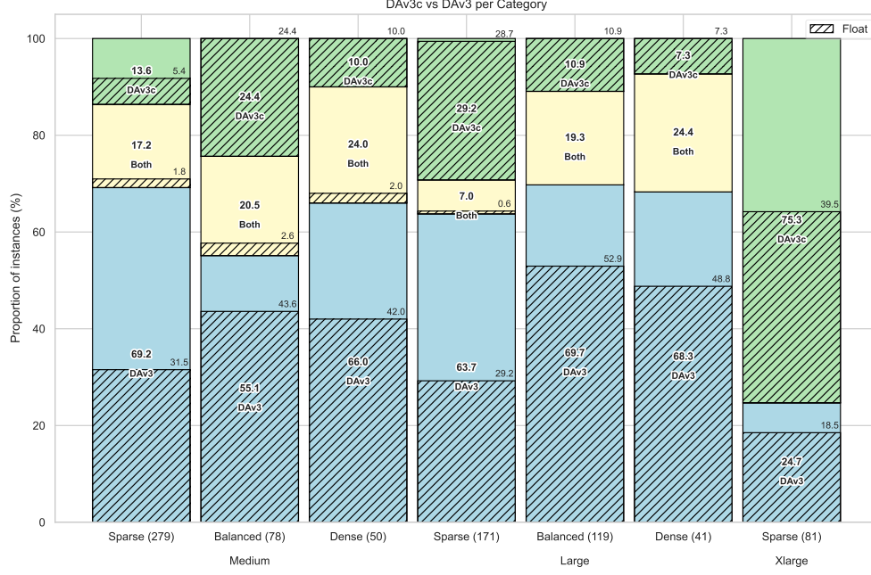
Fig. 4: Performance comparison between DAv3c and DAv3 across size–density groups using the same visualization scheme as Figure 2.
