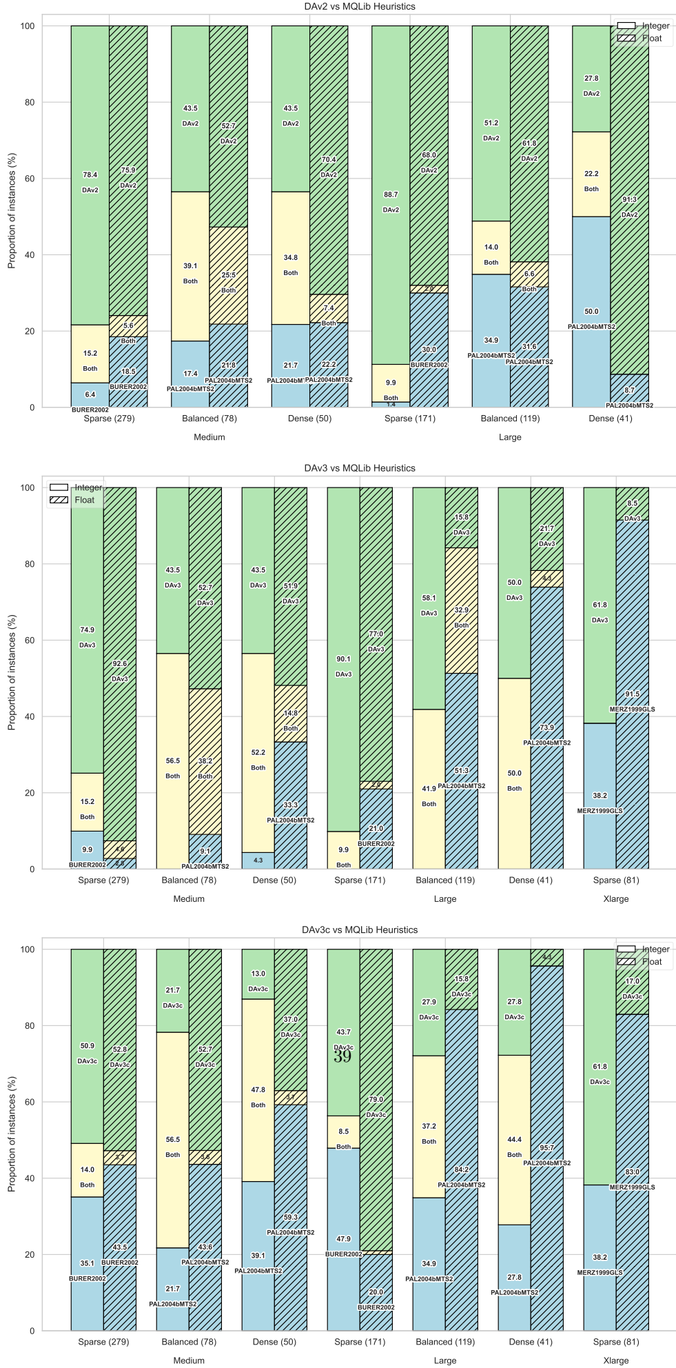
Fig. K7: Win-tie-loss distributions of DAV2, DAV3, and DAV3c against the MQLib heuristics on integer and float-weighted instances across the size-density categories
