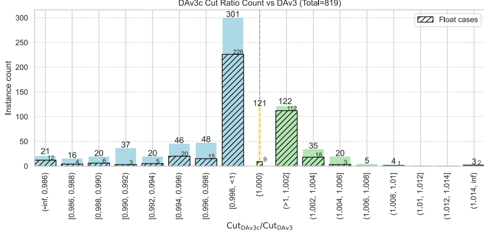
Fig. G5: Distribution of cut-value ratios for DAv3c relative to DAv3 using the same ratio definition as Figure 3.
