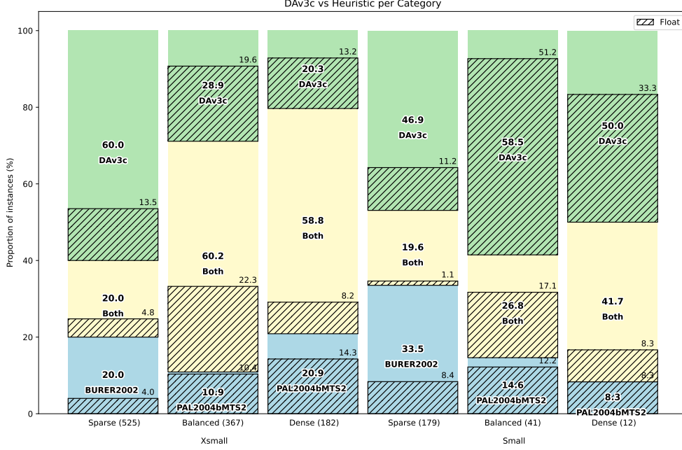
Fig. D4: Performance comparison between DAv3c and the category-selected MQLib heuristics for xsmall and small instances using the same visualization scheme as Figure 2.
